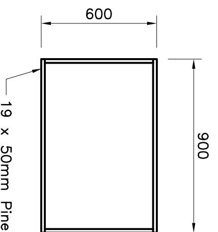
Part B Table Top Frame
