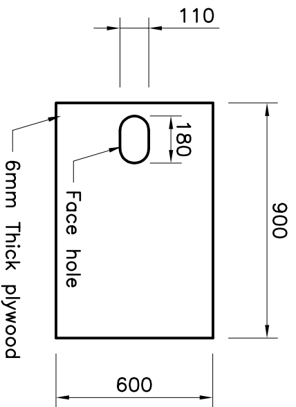
Part A Table Top
