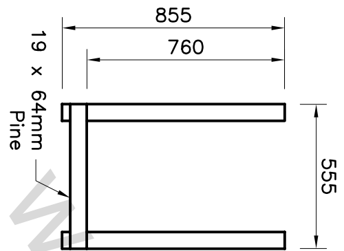
Part A Table Top
