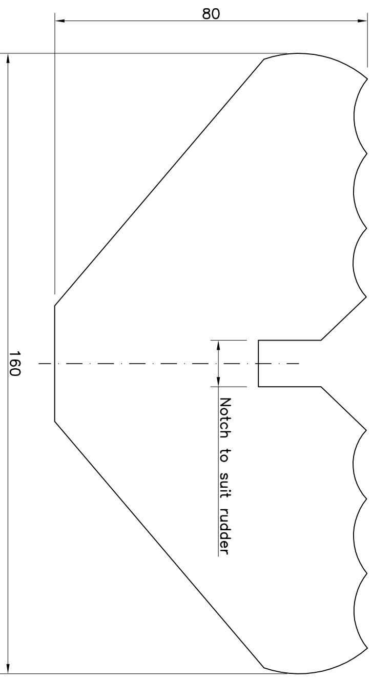
Full Size Tailplane Outline Alternate
