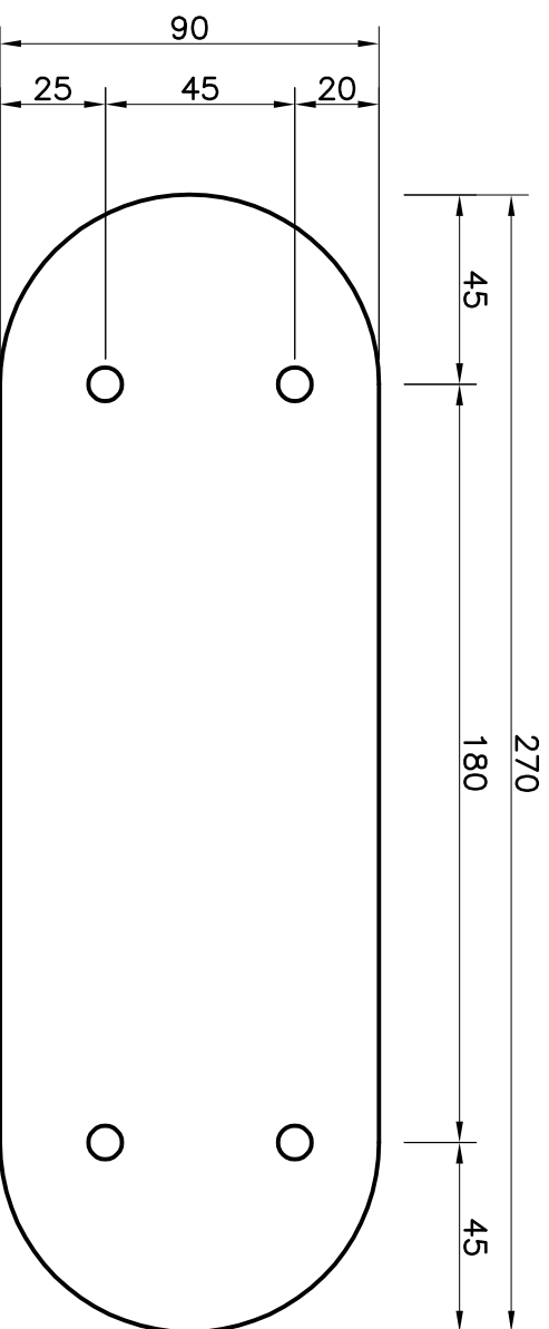
Bottom Wing
